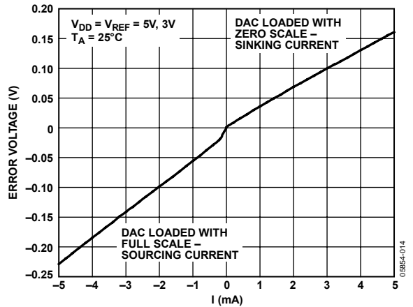
Figure 9. Headroom at Rails vs. Source and Sink Current
