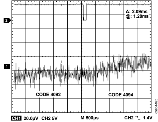
Figure 33. DAC Output with 50 Hz Filter on Output
