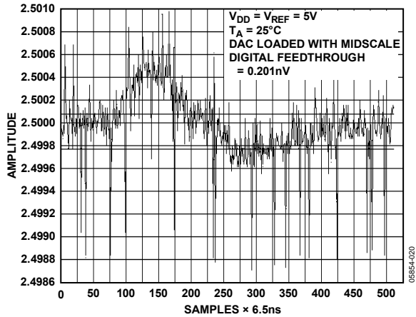
Figure 17. Digital Feedthrough
