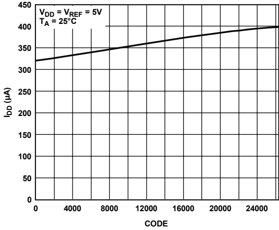
Figure 10. Supply Current vs. Code
