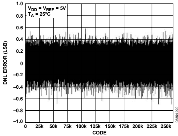
Figure 5. Typical DNL Plot in 50 Hz System Bandwidth
